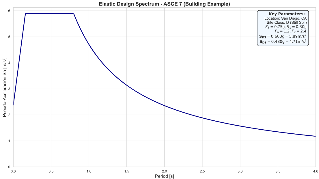
Figure C.1: Elastic Design Spectrum according to ASCE 7 for the case study site.
