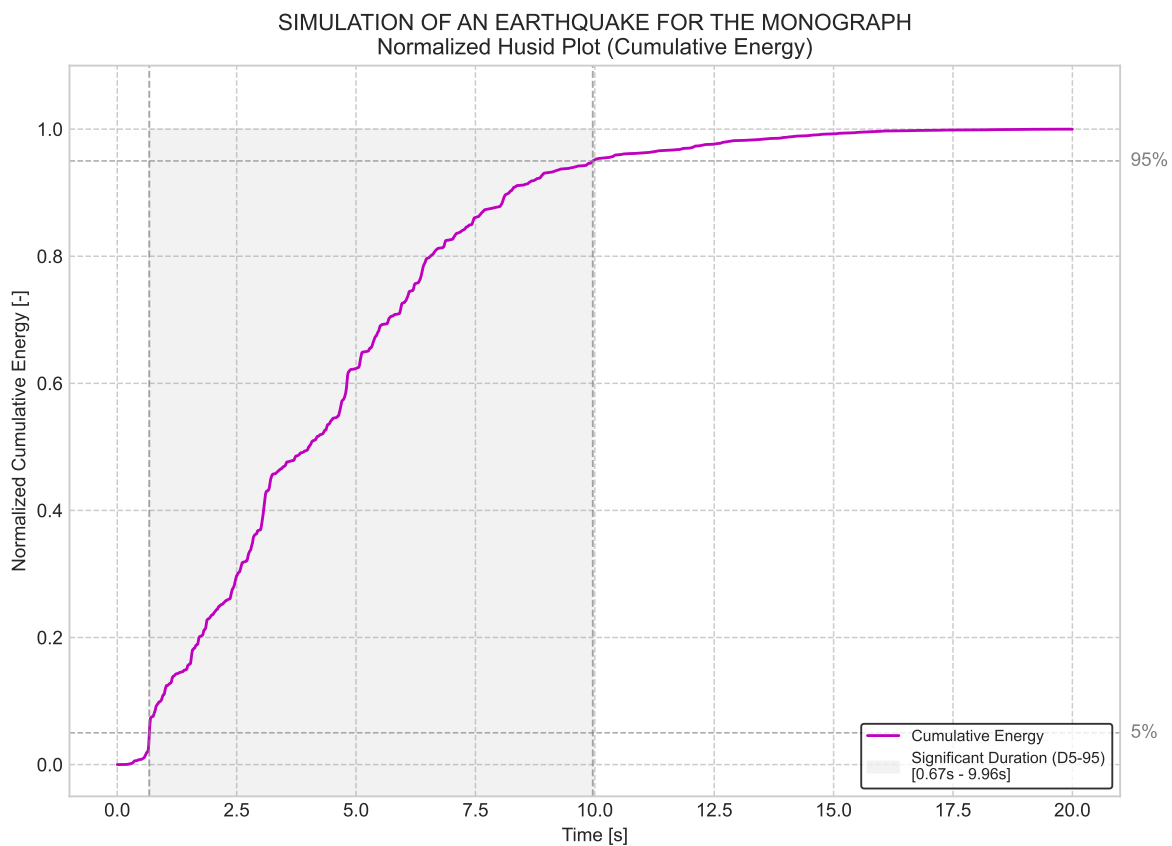
Figure 5.14: Example of the Normalized Husid Plot, showing the progressive accumulation of energy. The horizontal lines mark the 5% and 95% thresholds used to define the Significant Duration.
