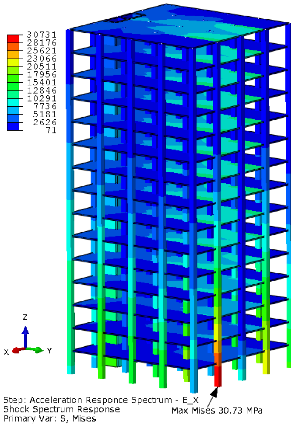
Figure C.16: Von Mises stress contour obtained from the Modal Response Spectrum Analysis (MRSA).
